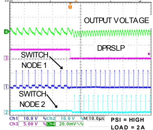
Figure 26. DPRSLP Transition
